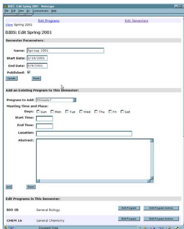
Figure 6: Example BIBS Database Editing Page
